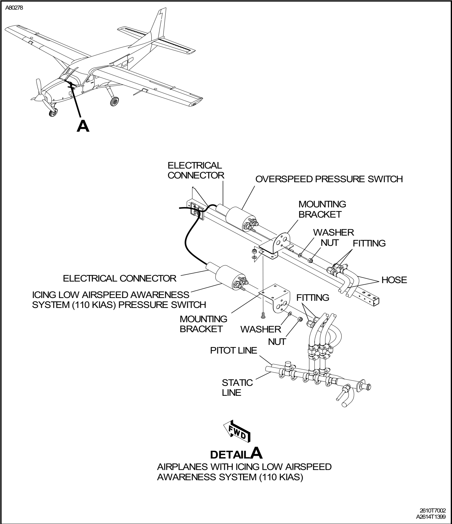
Figure 201 : Sheet 1 : LAA System Installation
